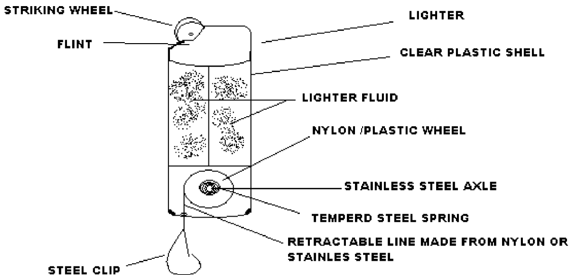
CLIP-ON RETRACTABLE LIGHTER
