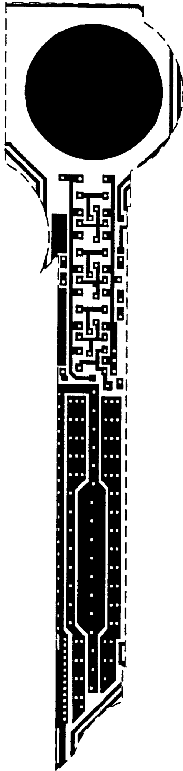
Metal 1 mask
