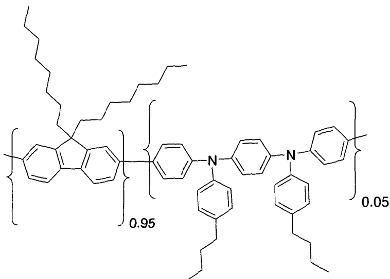
F8-PFB (2)
