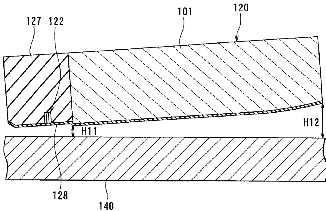
FIG. 43 RELATED ART
