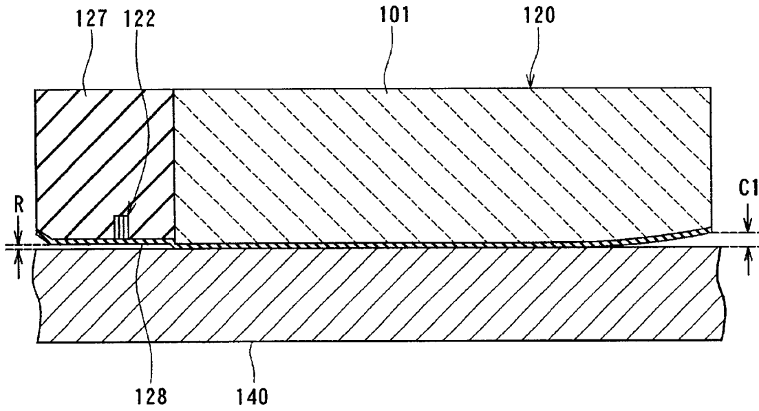
FIG. 40 RELATED ART
