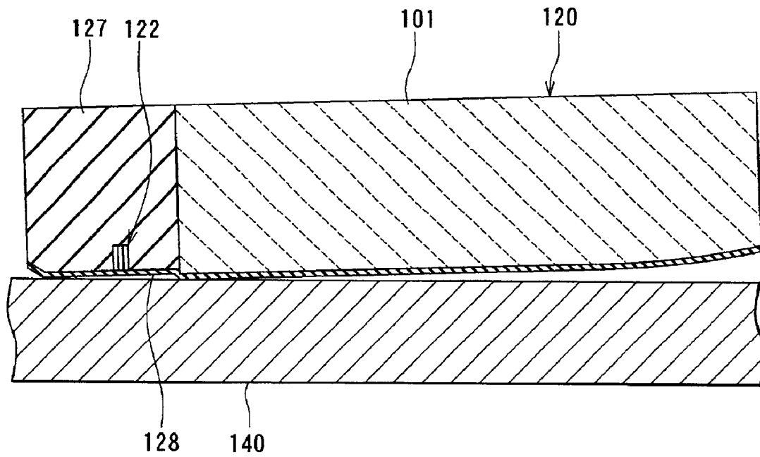
FIG. 42 RELATED ART
