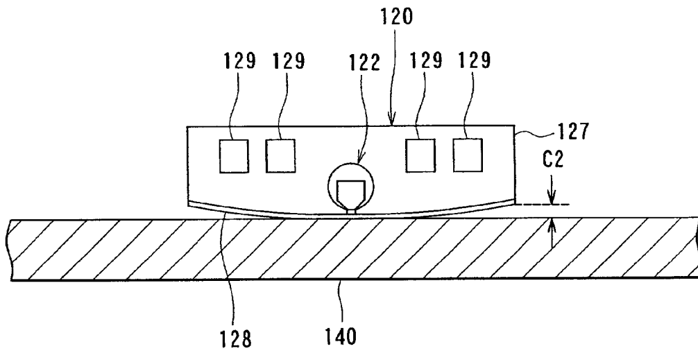
FIG. 40 RELATED ART
