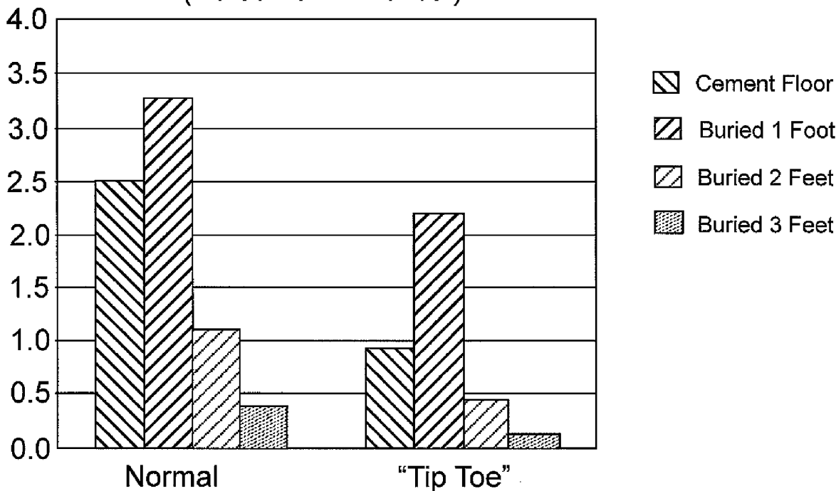
Ribbon Signal with Walking Over Ribbon (Person 6'2" 270 lbs.)
