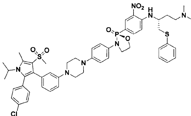
(S)-3-(4-(4-(3-(2-(4-chlorophenyl)-1-isopropyl-5-methyl-4-(methylsulfonyl)-1H-pyrrol-3-yl)phenyl)piperazin-1-yl)phenyl)-2-(4-(((R)-4-(dimethylamino)-1-(phenylthio)butan-2-yl)amino)-3-nitrophenyl)-1,3,2-oxazaphospholidine 2-oxide
