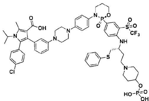
5-(4-chlorophenyl)-1-isopropyl-2-methyl-4-(3-(4-(4-((R)-2-oxido-2-(4-(((R)-1-(phenylthio)-4-(4-(phosphonooxy)piperidin-1-yl)butan-2-yl)amino)-3-((trifluoromethyl)sulfonyl)phenyl)-1,3,2-oxazaphosphinan-3-yl)phenyl)piperazin-1-yl)phenyl)-1H-pyrrole-3-carboxylic acid
