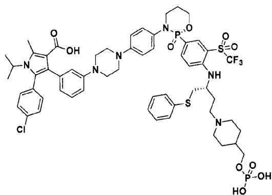
5-(4-chlorophenyl)-1-isopropyl-2-methyl-4-(3-(4-(4-((S)-2-oxido-2-(4-(((R)-1-(phenylthio)-4-(4-(phosphonooxy)methyl)piperidin-1-yl)butan-2-yl)amino)-3-((trifluoromethyl)sulfonyl)phenyl)-1,3,2-oxazaphosphinan-3-yl)phenyl)piperazin-1-yl)phenyl)-1H-pyrrole-3-carboxylic acid
