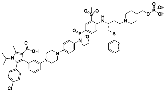
5-(4-chlorophenyl)-1-isopropyl-2-methyl-4-(3-(4-(4-((R)-2-(3-(methylsulfonyl)-4-(((R)-1-(phenylthio)-4-(4-((phosphonoxy)methyl)piperidin-1-yl)butan-2-yl)amino)phenyl)-2-oxido-1,3,2-oxazaphospholidin-3-yl)phenyl)piperazin-1-yl)phenyl)-1H-pyrrole-3-carboxylic acid
