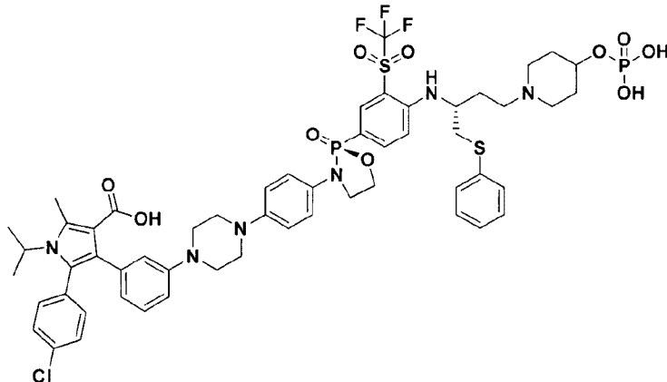
5-(4-chlorophenyl)-1-isopropyl-2-methyl-4-(3-(4-(4-(((S)-2-oxido-2-(4-(((R)-1-(phenylthio)-4-(4-(phosphonooxy)piperidin-1-yl)butan-2-yl)amino)-3-((trifluoromethyl)sulfonyl)phenyl)-1,3,2-oxazaphospholidin-3-yl)phenyl)piperazin-1-yl)phenyl)-1H-pyrrole-3-carboxylic acid
