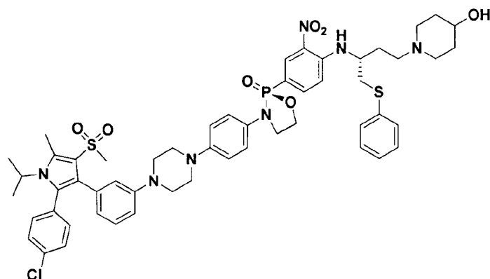
(S)-3-(4-(4-(3-(2-(4-chlorophenyl)-1-isopropyl-5-methyl-4-(methylsulfonyl)-1H-pyrrol-3-yl)phenyl)piperazin-1-yl)phenyl)-2-(4-(((R)-4-(4-hydroxypiperidin-1-yl)-1-(phenylthio)butan-2-yl)amino)-3-nitrophenyl)-1,3,2-oxazaphospholidine 2-oxide
