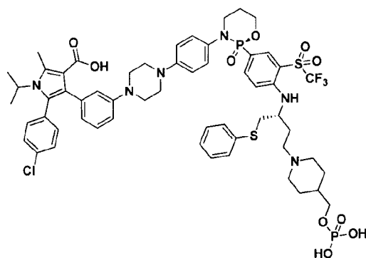
5-(4-chlorophenyl)-1-isopropyl-2-methyl-4-(3-(4-(4-((R)-2-oxido-2-(4-(((R)-1-(phenylthio)-4-(4-(phosphonooxy)methyl)piperidin-1-yl)butan-2-yl)amino)-3-((trifluoromethyl)sulfonyl)phenyl)-1,3,2-oxazaphosphinan-3-yl)phenyl)piperazin-1-yl)phenyl)-1H-pyrrole-3-carboxylic acid
