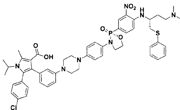
5-(4-chlorophenyl)-4-(3-(4-(4-(((R)-2-(4-(((R)-4-(dimethylamino)-1-(phenylthio)butan-2-yl)amino)-3-nitrophenyl)-2-oxido-1,3,2-oxazaphospholidin-3-yl)phenyl)piperazin-1-yl)phenyl)-1-isopropyl-2-methyl-1H-pyrrole-3-carboxylic acid
