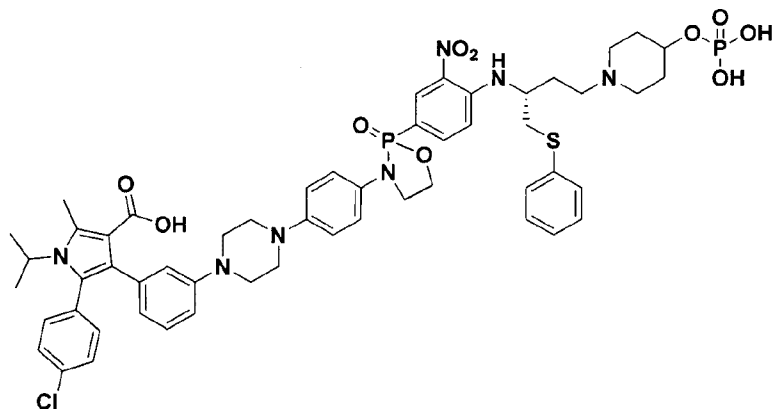
5-(4-chlorophenyl)-1-isopropyl-2-methyl-4-(3-(4-(4-(2-(3-nitro-4-(((R)-1-(phenylthio)-4-(4-(phosphonoxy)piperidin-1-yl)butan-2-yl)amino)phenyl)-2-oxido-1,3,2-oxazaphospholidin-3-yl)phenyl)piperazin-1-yl)phenyl)-1H-pyrrole-3-carboxylic acid
