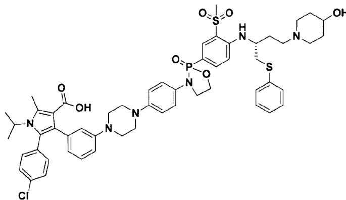
5-(4-chlorophenyl)-4-(3-(4-(4-(2-(4-(((R)-4-(4-hydroxypiperidin-1-yl)-1-(phenylthio)butan-2-yl)amino)-3-(methylsulfonyl)phenyl)-2-oxido-1,3,2-oxazaphospholidin-3-yl)phenyl)piperazin-1-yl)phenyl)-1-isopropyl-2-methyl-1H-pyrrole-3-carboxylic acid
