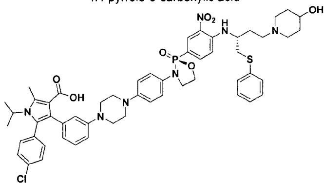
5-(4-chlorophenyl)-4-(3-(4-(4-(((S)-2-(4-(((R)-4-(4-hydroxypiperidin-1-yl)-1-(phenylthio)butan-2-yl)amino)-3-nitrophenyl)-2-oxido-1,3,2-oxazaphospholidin-3-yl)phenyl)piperazin-1-yl)phenyl)-1-isopropyl-2-methyl-1H-pyrrole-3-carboxylic acid
