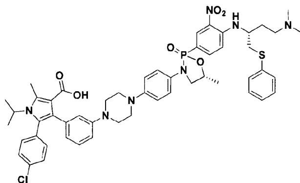
5-(4-chlorophenyl)-4-(3-(4-(4-((5R)-2-(4-(((R)-4-(dimethylamino)-1-(phenylthio)butan-2-yl)amino)-3-nitrophenyl)-5-methyl-2-oxido-1,3,2-oxazaphospholidin-3-yl)phenyl)piperazin-1-yl)phenyl)-1-isopropyl-2-methyl-1H-pyrrole-3-carboxylic acid
