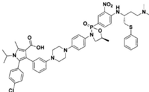
5-(4-chlorophenyl)-4-(3-(4-(4-((5S)-2-(4-(((R)-4-(dimethylamino)-1-(phenylthio)butan-2-yl)amino)-3-nitrophenyl)-5-methyl-2-oxido-1,3,2-oxazaphospholidin-3-yl)phenyl)piperazin-1-yl)phenyl)-1-isopropyl-2-methyl-1H-pyrrole-3-carboxylic acid
