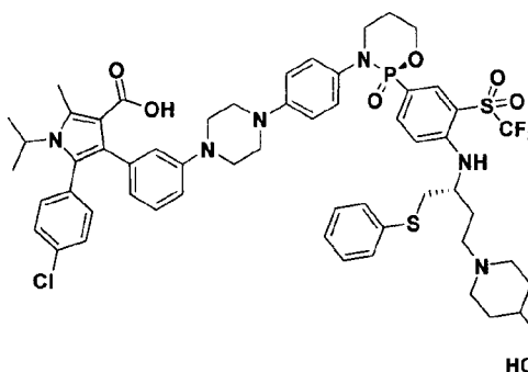
5-(4-chlorophenyl)-4-(3-(4-(4-((R)-2-(4-(((R)-4-(4-(hydroxymethyl)piperidin-1-yl)-1-(phenylthio)butan-2-yl)amino)-3-((trifluoromethyl)sulfonyl)phenyl)-2-oxido-1,3,2-oxazaphosphinan-3-yl)phenyl)piperazin-1-yl)phenyl)-1-isopropyl-2-methyl-1H-pyrrole-3-carboxylic acid
