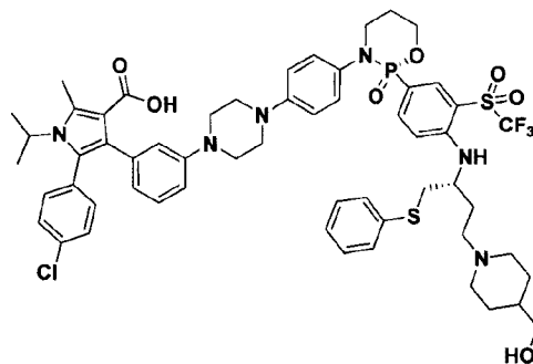
5-(4-chlorophenyl)-4-(3-(4-(4-((S)-2-(4-(((R)-4-(4-(hydroxymethyl)piperidin-1-yl)-1-(phenylthio)butan-2-yl)amino)-3-((trifluoromethyl)sulfonyl)phenyl)-2-oxido-1,3,2-oxazaphosphinan-3-yl)phenyl)piperazin-1-yl)phenyl)-1-isopropyl-2-methyl-1H-pyrrole-3-carboxylic acid
