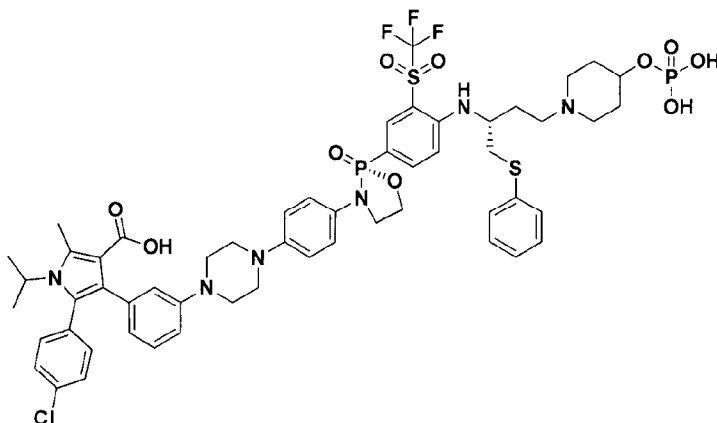
5-(4-chlorophenyl)-1-isopropyl-2-methyl-4-(3-(4-(4-(((S)-2-oxido-2-(4-(((R)-1-(phenylthio)-4-(4-(phosphonooxy)piperidin-1-yl)butan-2-yl)amino)-3-((trifluoromethyl)sulfonyl)phenyl)-1,3,2-oxazaphospholidin-3-yl)phenyl)piperazin-1-yl)phenyl)-1H-pyrrole-3-carboxylic acid
