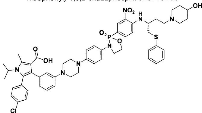
5-(4-chlorophenyl)-4-(3-(4-(4-(2-(4-(((R)-4-(4-hydroxypiperidin-1-yl)-1-(phenylthio)butan-2-yl)amino)-3-nitrophenyl)-2-oxido-1,3,2-oxazaphospholidin-3-yl)phenyl)piperazin-1-yl)phenyl)-1-isopropyl-2-methyl-1H-pyrrole-3-carboxylic acid
