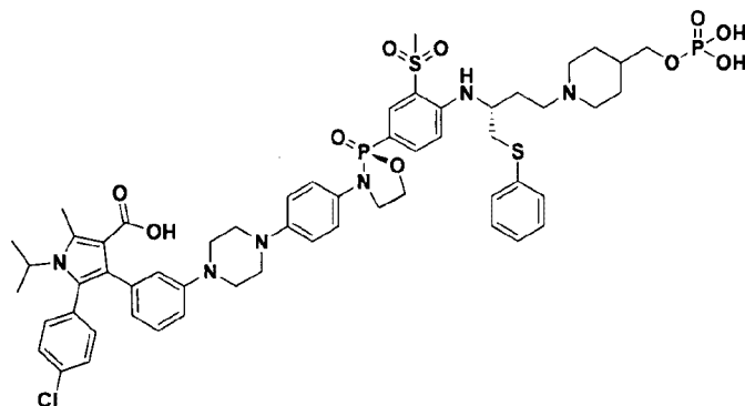
5-(4-chlorophenyl)-1-isopropyl-2-methyl-4-(3-(4-(4-((S)-2-(3-(methylsulfonyl)-4-(((R)-1-(phenylthio)-4-(4-((phosphonoxy)methyl)piperidin-1-yl)butan-2-yl)amino)phenyl)-2-oxido-1,3,2-oxazaphospholidin-3-yl)phenyl)piperazin-1-yl)phenyl)-1H-pyrrole-3-carboxylic acid
