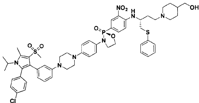
(S)-3-(4-(4-(3-(2-(4-chlorophenyl)-1-isopropyl-5-methyl-4-(methylsulfonyl)-1H-pyrrol-3-yl)phenyl)piperazin-1-yl)phenyl)-2-(4-(((R)-4-(4-(hydroxymethyl)piperidin-1-yl)-1-(phenylthio)butan-2-yl)amino)-3-nitrophenyl)-1,3,2-oxazaphospholidine 2-oxide
