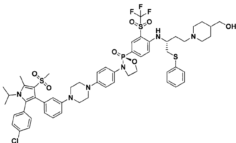
(S)-3-(4-(4-(3-(2-(4-chlorophenyl)-1-isopropyl-5-methyl-4-(methylsulfonyl)-1H-pyrrol-3-yl)phenyl)piperazin-1-yl)phenyl)-2-(4-(((R)-4-(4-(hydroxymethyl)piperidin-1-yl)-1-(phenylthio)butan-2-yl)amino)-3-((trifluoromethyl)sulfonyl)phenyl)-1,3,2-oxazaphospholidine 2-oxide
