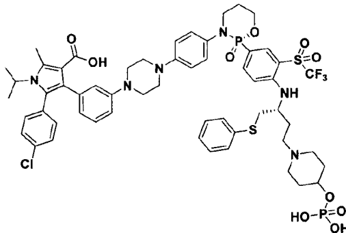
5-(4-chlorophenyl)-1-isopropyl-2-methyl-4-(3-(4-(4-((S)-2-oxido-2-(4-(((R)-1-(phenylthio)-4-(4-(phosphonoxy)piperidin-1-yl)butan-2-yl)amino)-3-((trifluoromethyl)sulfonyl)phenyl)-1,3,2-oxazaphosphinan-3-yl)phenyl)piperazin-1-yl)phenyl)-1H-pyrrole-3-carboxylic acid
