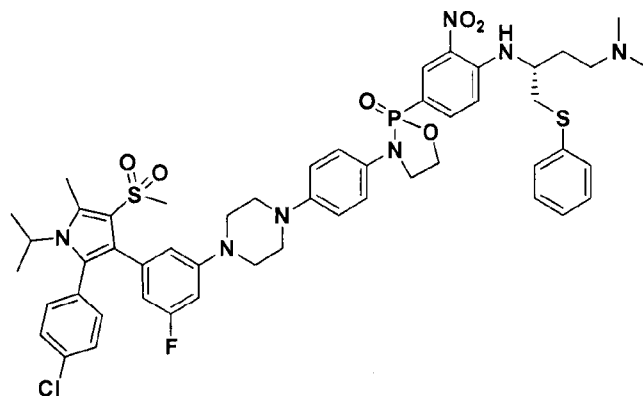
3-(4-(4-(3-(2-(4-chlorophenyl)-1-isopropyl-5-methyl-4-(methylsulfonyl)-1H-pyrrol-3-yl)-5-fluorophenyl)piperazin-1-yl)phenyl)-2-(4-(((R)-4-(dimethylamino)-1-(phenylthio)butan-2-yl)amino)-3-nitrophenyl)-1,3,2-oxazaphospholidine 2-oxide
