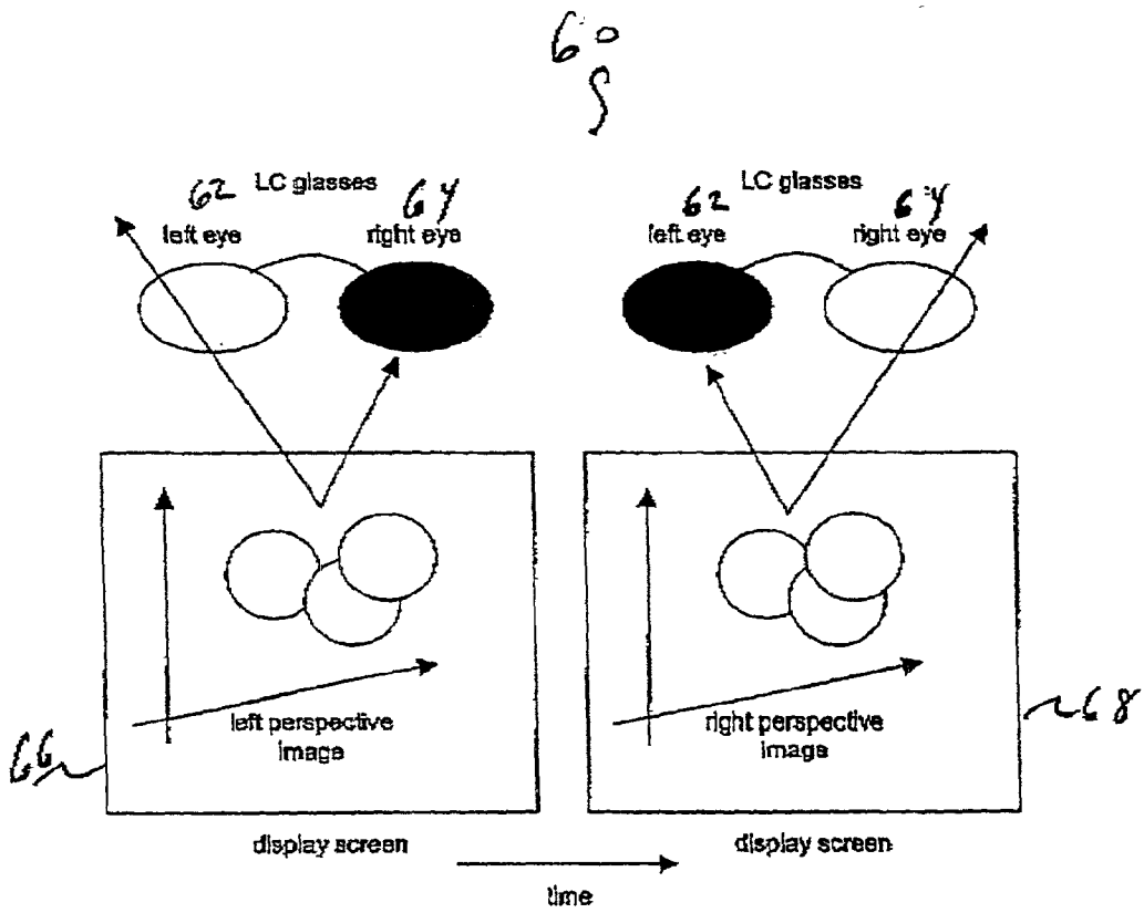
Figure 5 Use of LC Shutter Glasses in Stereoscopic Visualization
