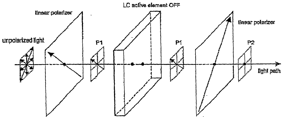
Figure 4 Diagram of Typical LC Shutter Operatio in OFF State
