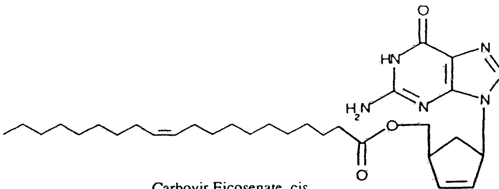
Carbovir Elaidate
