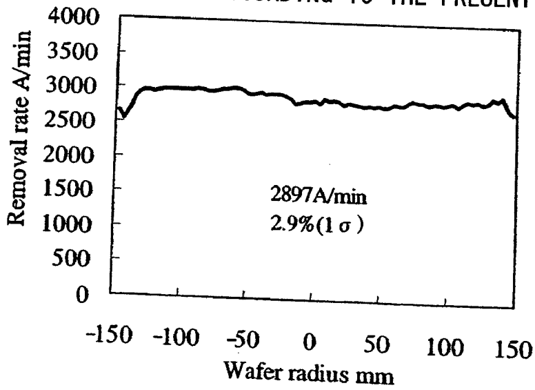
RESULT OF POLISHING ACCORDING TO THE PRESENT INVENTION
