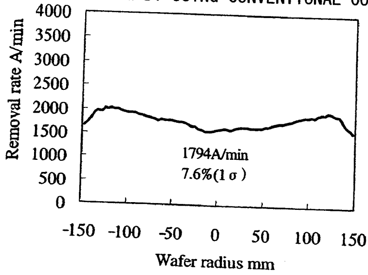
RESULT OF POLISHING BY USING CONVENTIONAL CONFIGURATION
