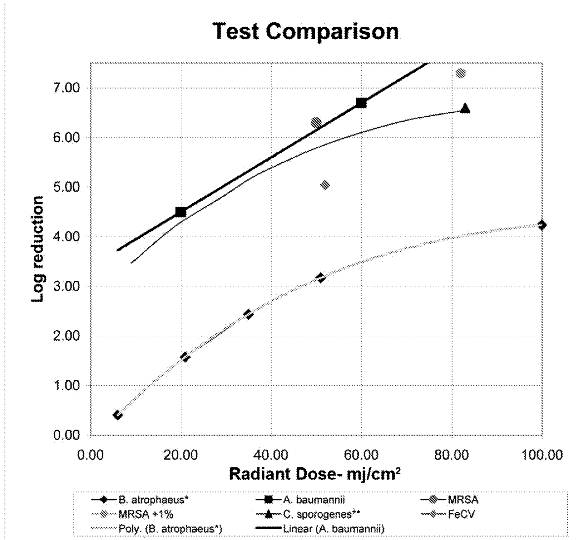
Figure 14: Sterilray Technology Test Data
