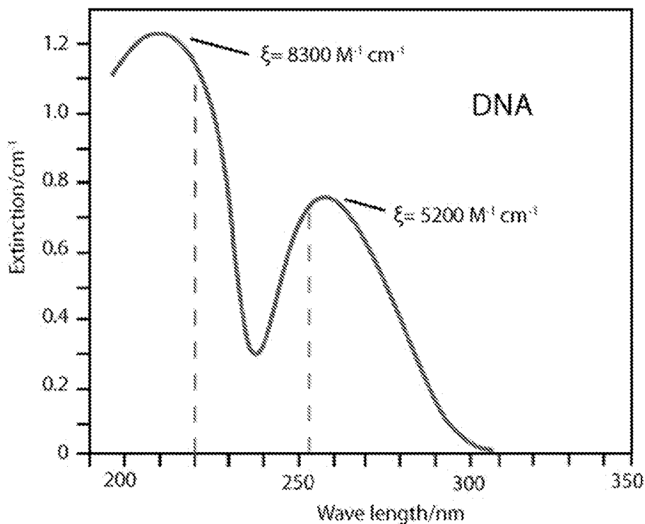
Figure 9: UV Absorption of DNA
