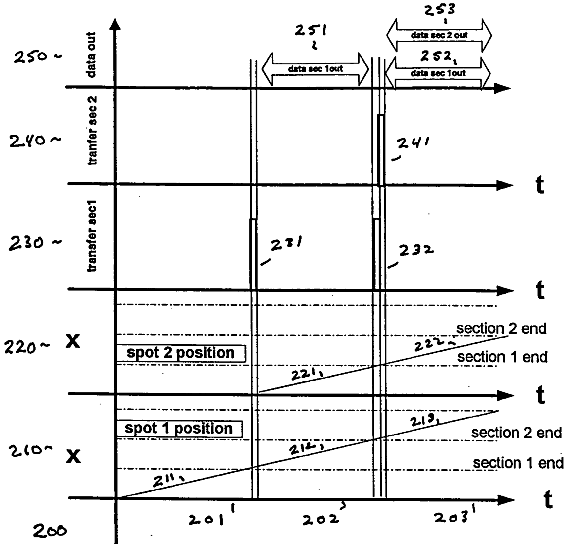
Figure 2: Timing diagram
