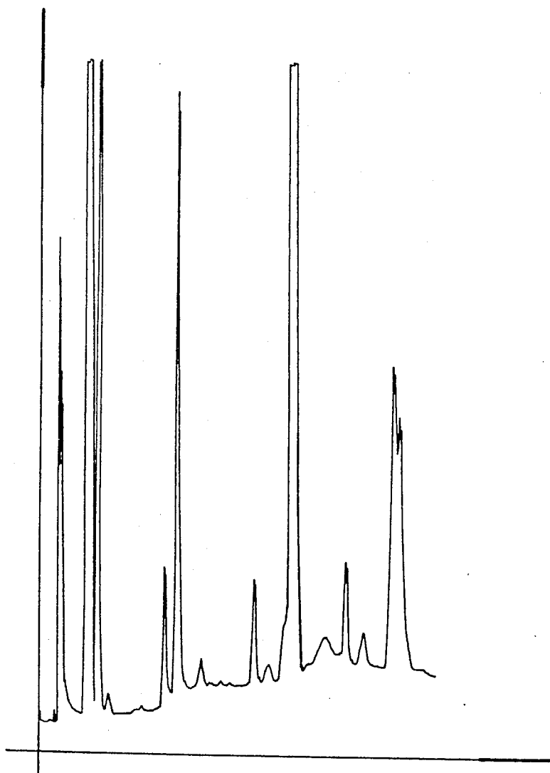
GLC PROFILE FOR EXAMPLE I.
