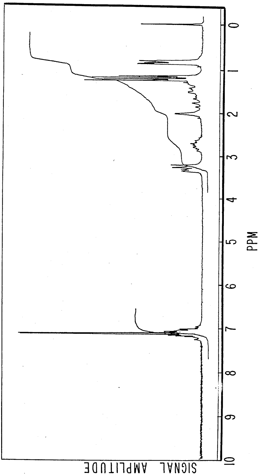
NMR SPECTRUM FOR EXAMPLE III
