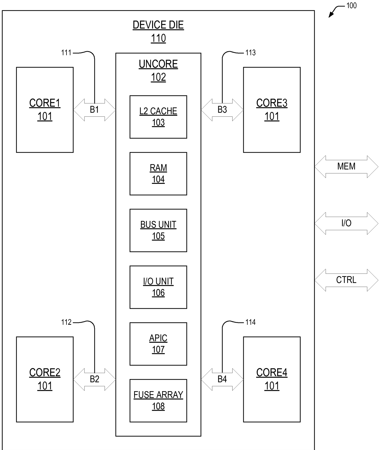
MULTI-CORE PROCESSOR WITH NON-CORE COMMON RESOURCES
