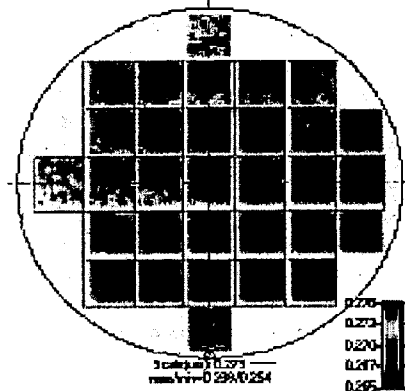
Resist thickness
