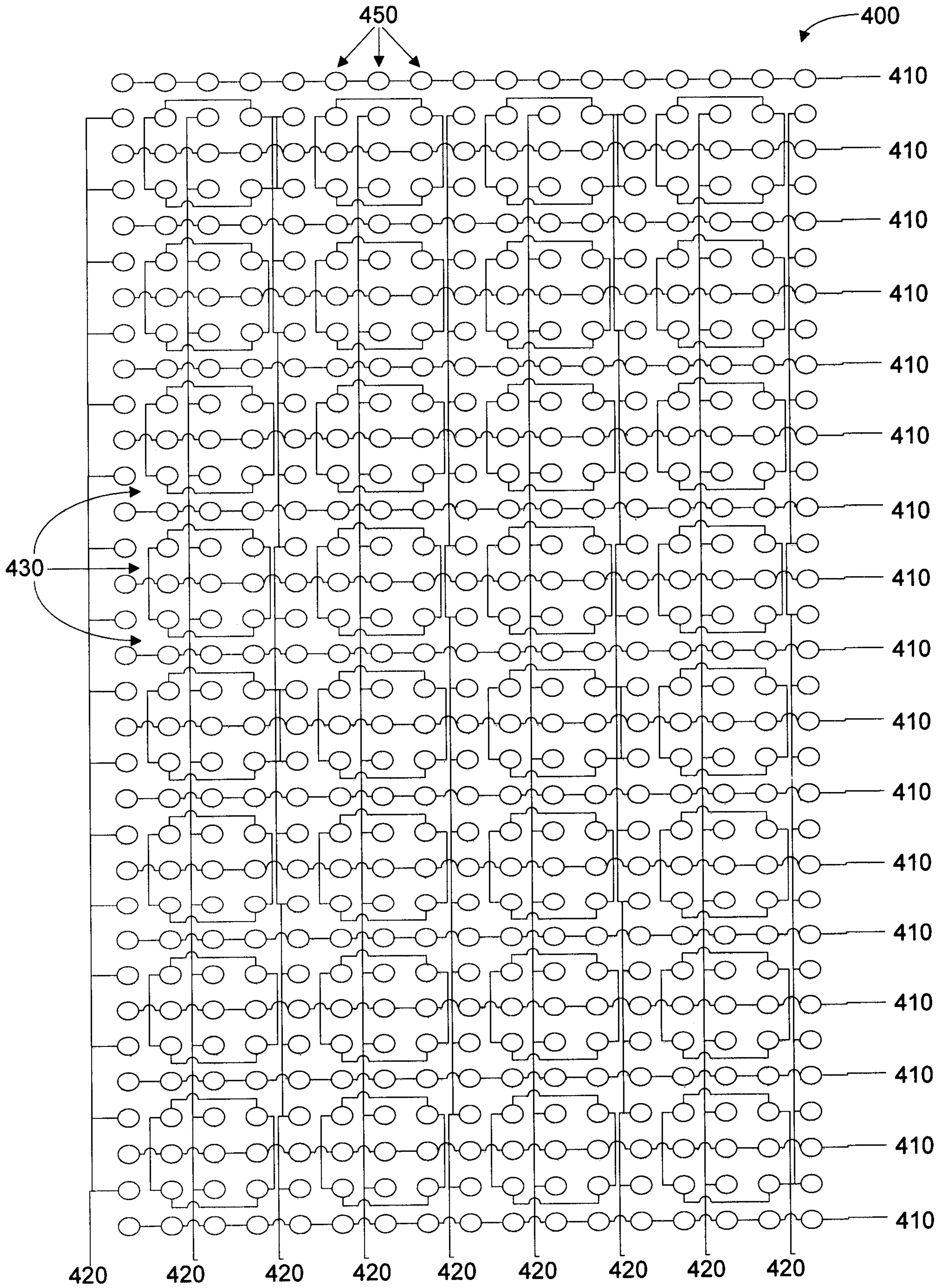
Schematic of Sensor Array
