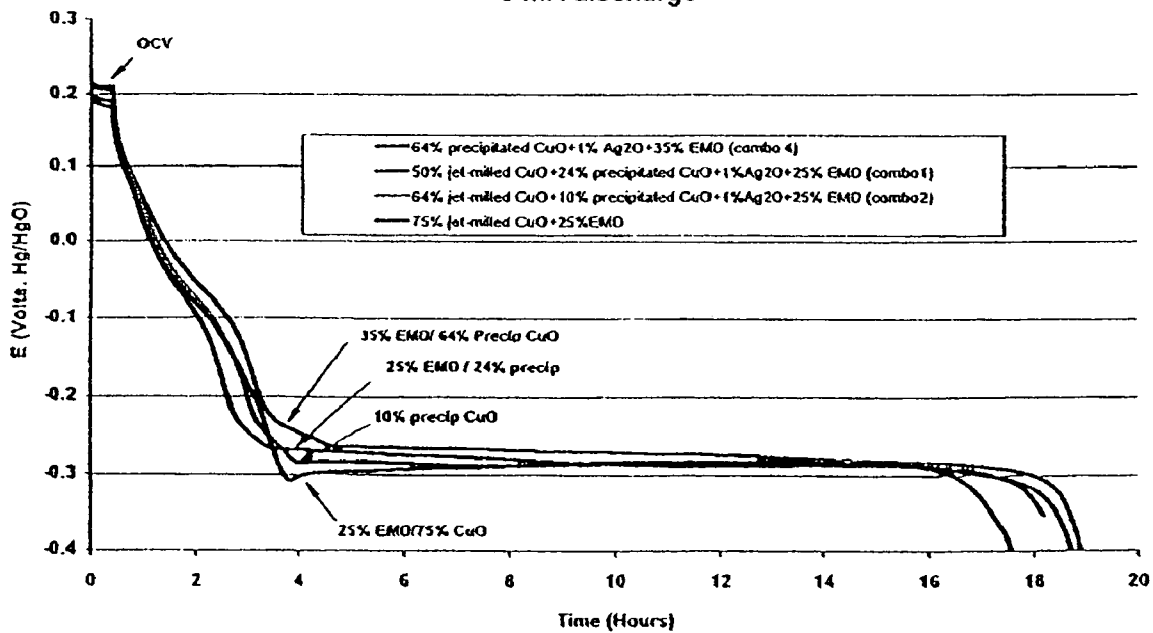
Smoothinging EMD/CuO transition by chemically precipitated CuO 5 mA discharge
