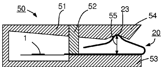
(side view along CC') FIG. 5B
