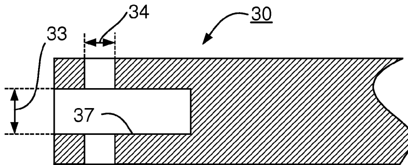
(side view along AA') FIG. 3C
