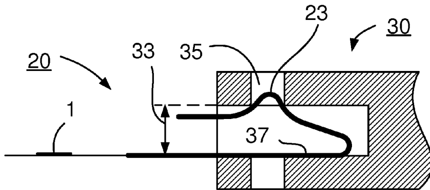
(Side view along BB') FIG. 4B
