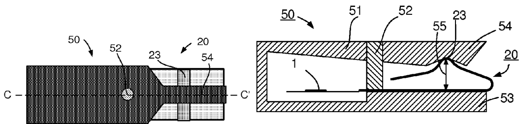
(top view) FIG. 5A
