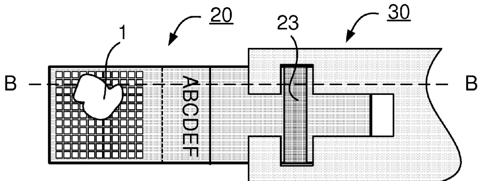
(top view) FIG. 4A
