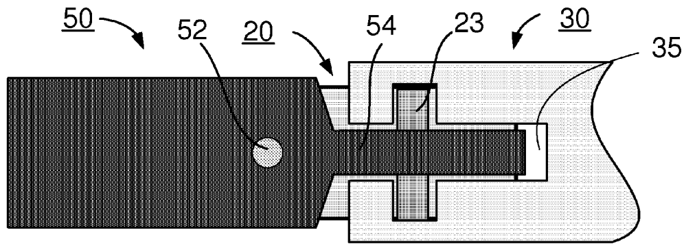
(top view) FIG. 6A
