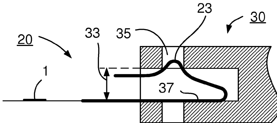
(Side view along BB')
