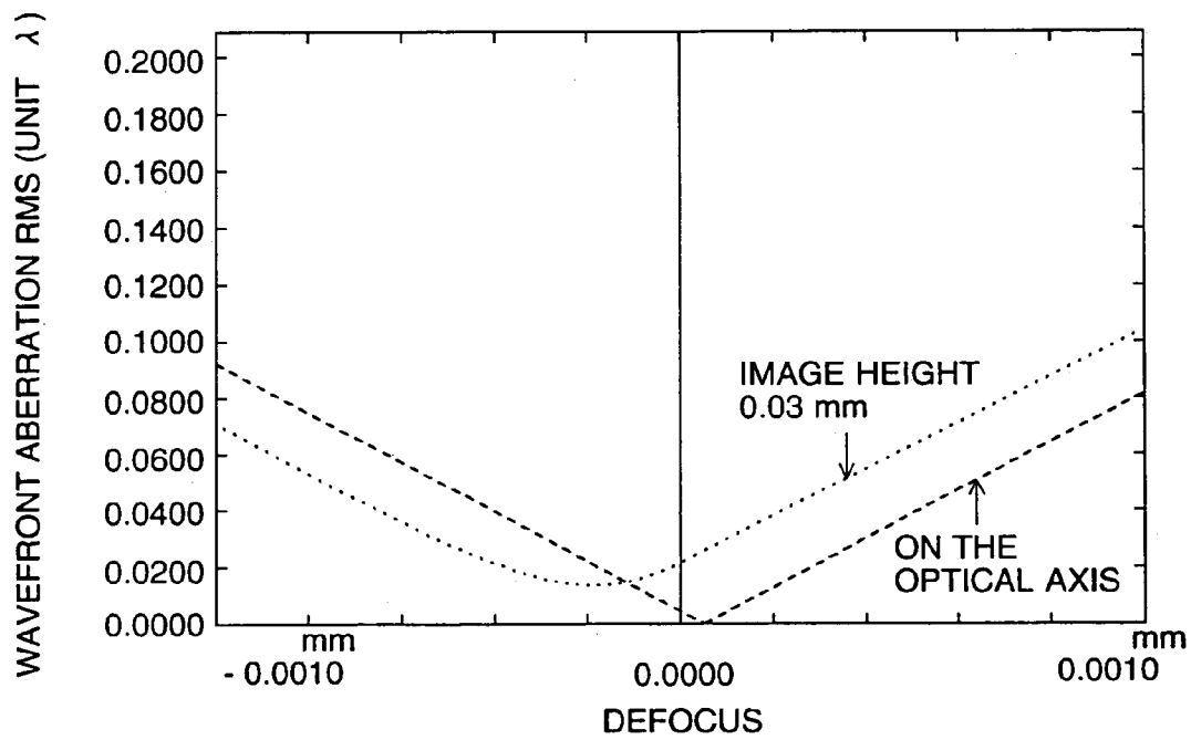
DIAGRAM SHOWING WAVEFRONT ABERRATION RMS FOR WAVELENGTH \lambda = 650\text{nm} IN EXAMPLE 6
