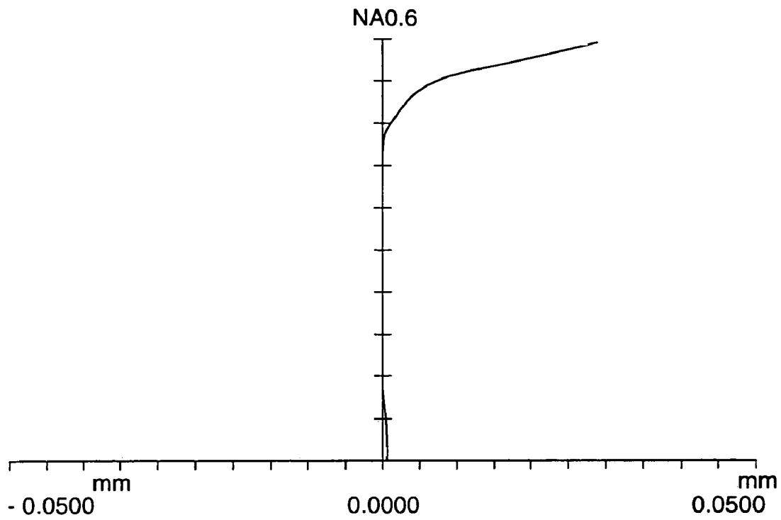
DIAGRAM SHOWING SPHERICAL ABERRATION FOR WAVELENGTH \lambda = 780\text{nm} IN EXAMPLE 6
