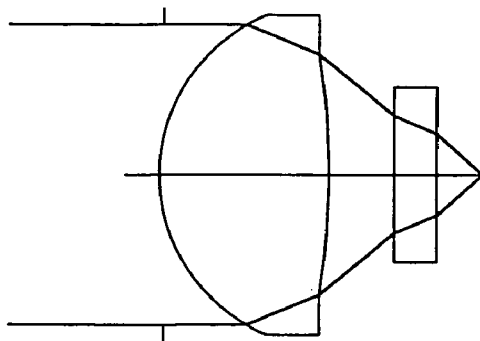
CROSS SECTIONAL VIEW OF OBJECTIVE LENS AND ILLUSTRATION SHOWING OPTICAL PATH FOR WAVELENGTH \lambda = 400\text{nm}
