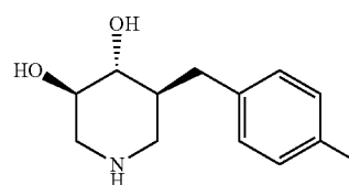
(3R,4R,5S)-5-(4-methylbenzyl)piperidine-3,4-diol
