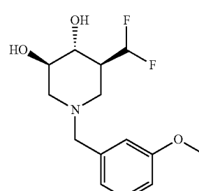
(3R,4R,5S)-5-(difluoromethyl)-1-(3-methoxybenzyl)piperidine-3,4-diol
