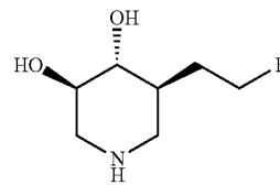
(3R,4R,5S)-5-(2-fluoroethyl)piperidine-3,4-diol
