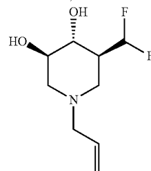
(3R,4R,5S)-1-allyl-5-(difluoromethyl)piperidine-3,4-diol
