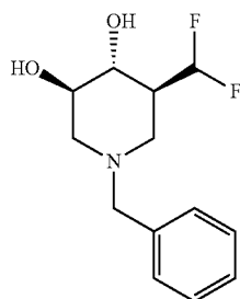
(3R,4R,5S)-1-benzyl-5-(difluoromethyl)piperidine-3,4-diol
