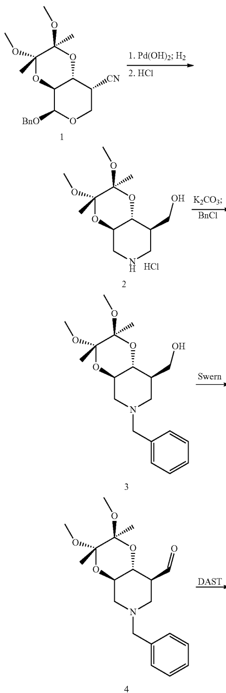
Scheme 3
