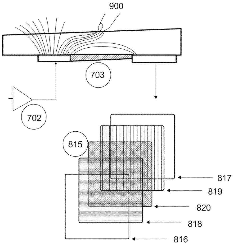
FIG. 4 (PRIOR ART)
