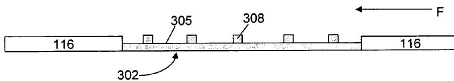
Fig. 3D (end view)
