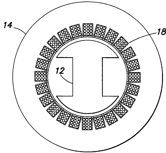
FIG. 1 (PRIOR ART)
