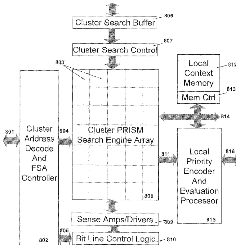
PRISM Memory Cluster Block Diagram
