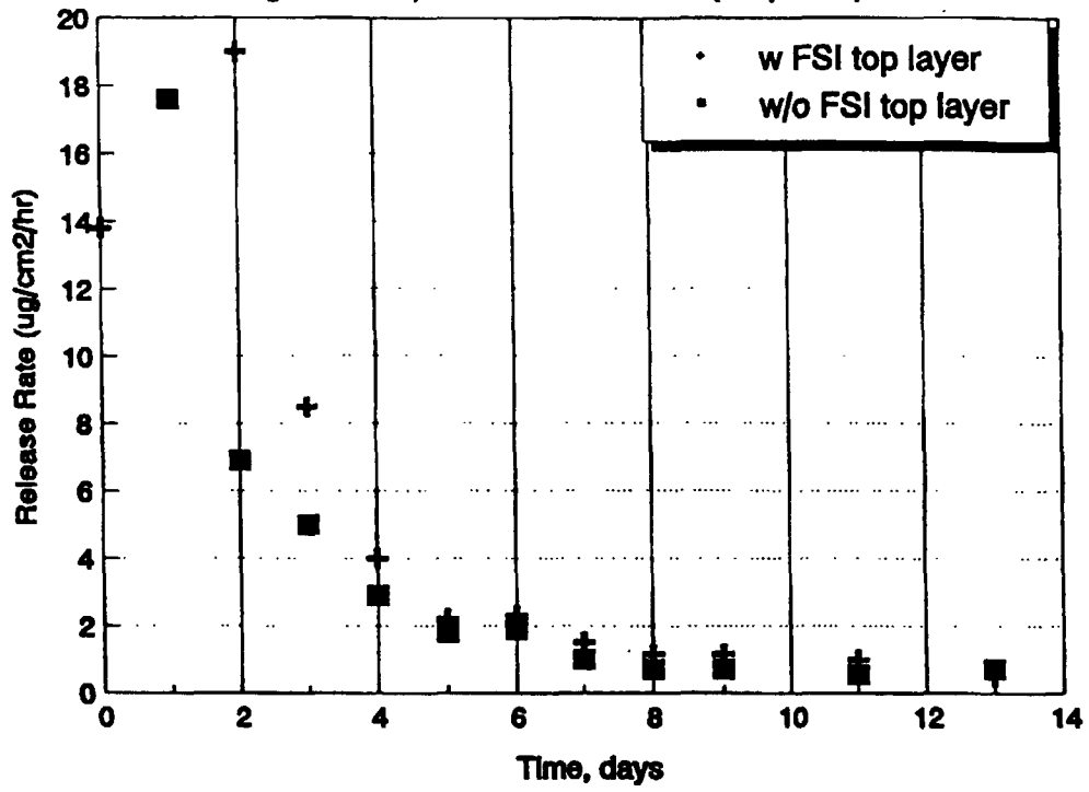
Figure 7. W or w/o fluorosilicone (FSI) top coat
