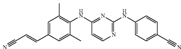
Compound 1 = (E); compound 10 = (Z)
