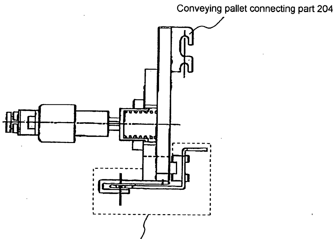
Fixing part of casting inlet part 202
