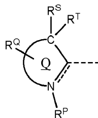
ligand A,
