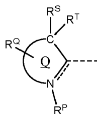
ligand A,
