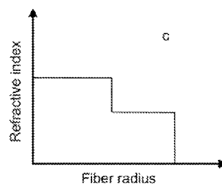
Single-mode multistep index (at least one step)
