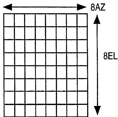
NORMAL BEAMFORMER
