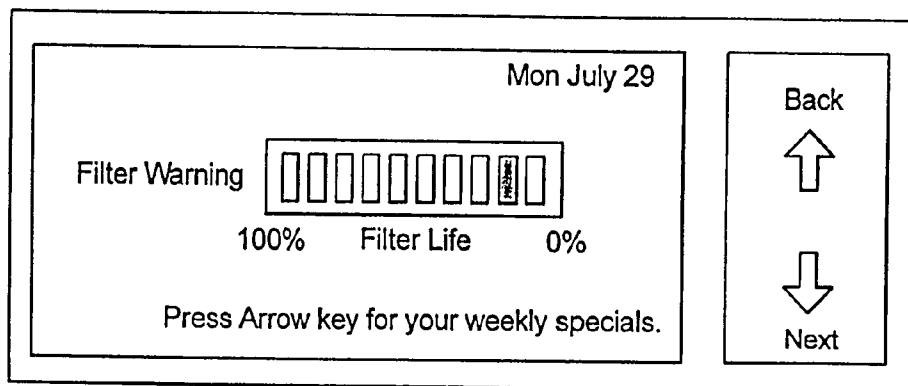
Deactivated Page
