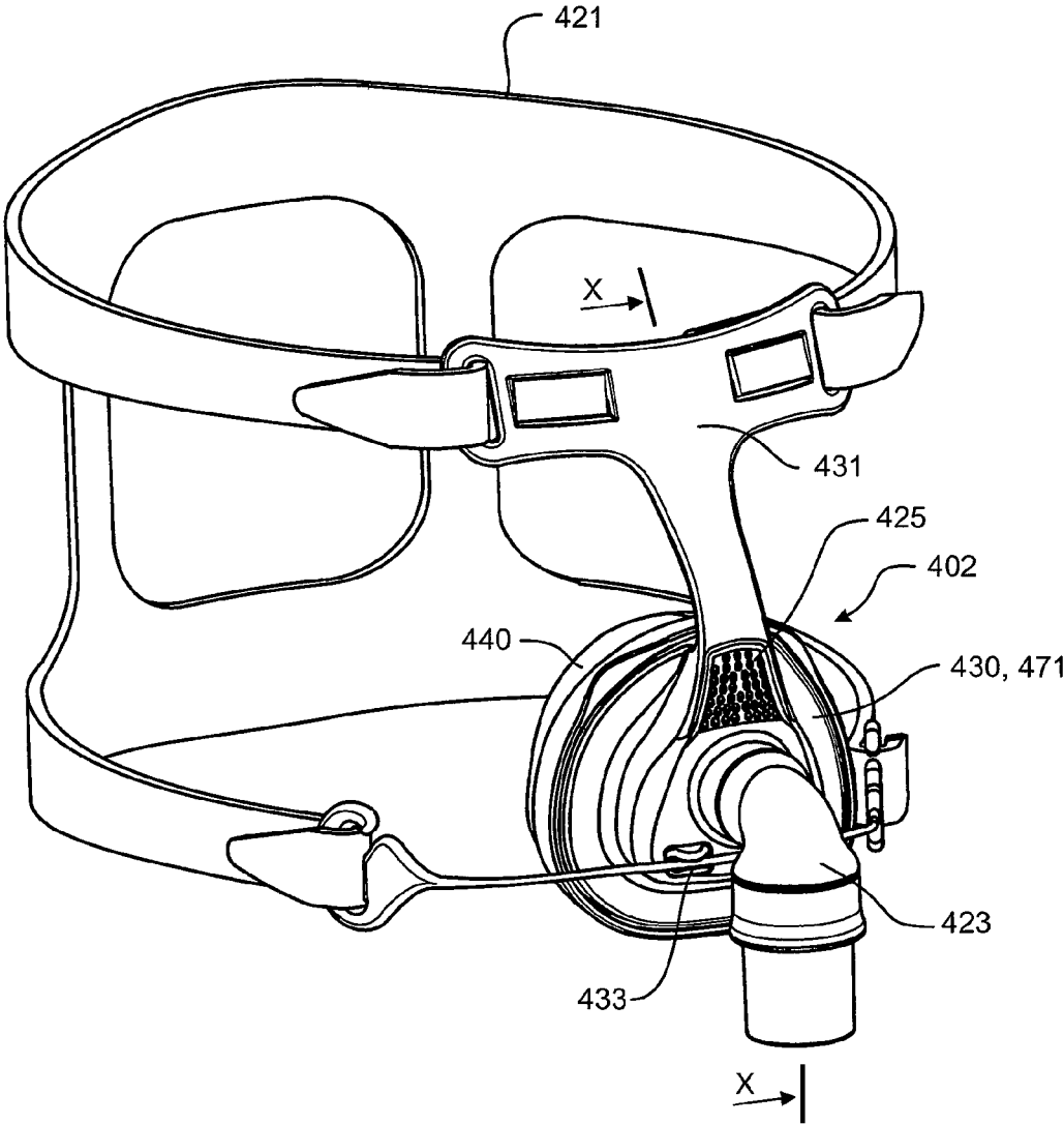
FIGURE 2 (Prior Art)
