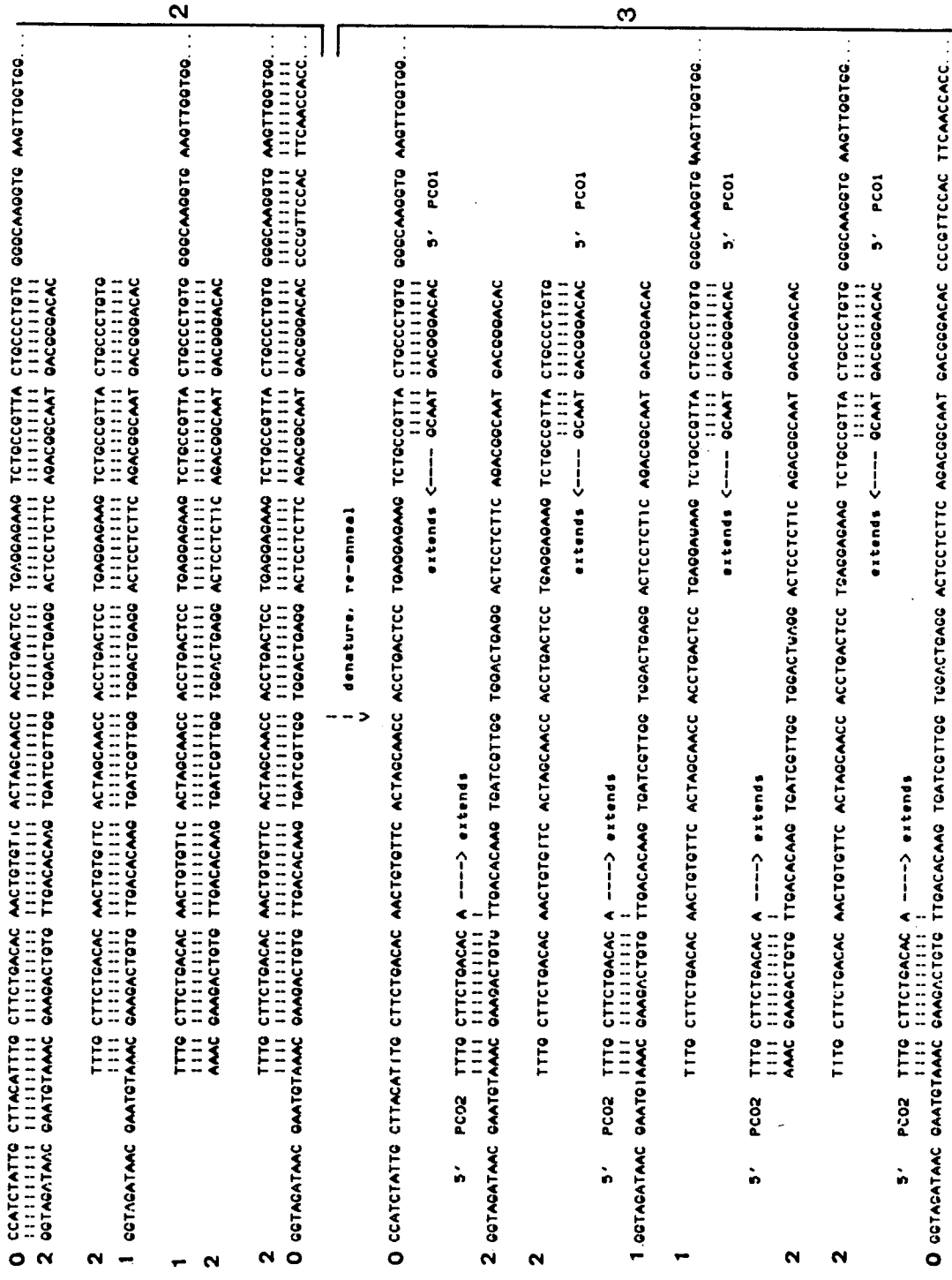
FIG.4-2 Polymerase, dNTPs
