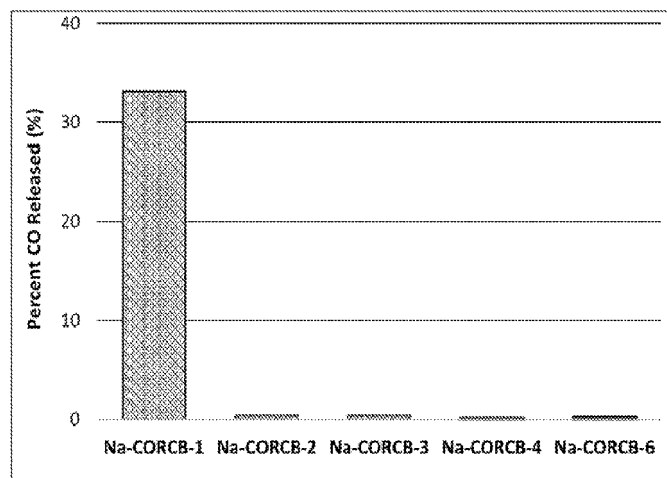
Figure 6. Percent CO released by sodium salts of CORCBs measured with CO meter. CORCB sodium salts were dissolved in H 2 O and incubated at 37°C for 24 hours. The head space air that contained CO gas is analyzed by CO meter and the ppm readings converted to the micromole amount for percent calculation.
