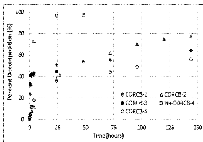
Figure 7. Percent decomposition of CORCBs in the presence of ROS monitored by ^1\text{H} NMR. CORCBs were dissolved in \text{H}_2\text{O} and 1.5 equivalents of \text{H}_2\text{O}_2 added before incubation in 37^\circ\text{C} . ^1\text{H} NMR spectra were taken at specified times to track the decomposition rates.
