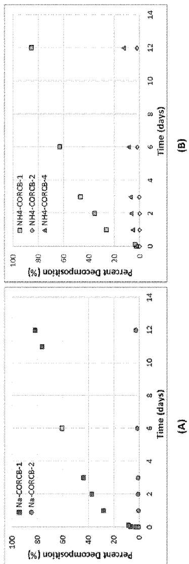
Figure 4. Auto-decomposition of CORCB salts monitored by 1 H NMR. (A) CORCB sodium salts and (B) CORCB ammonium salts. All CORCB salts are soluble in D 2 O solvent. After incubation at 37°C, 1 H NMR spectra were taken at specified times to track the decomposition rates. Sodium salts of CORCB-3, 4, and 5 had insignificant amounts of decomposition, therefore data not shown.
