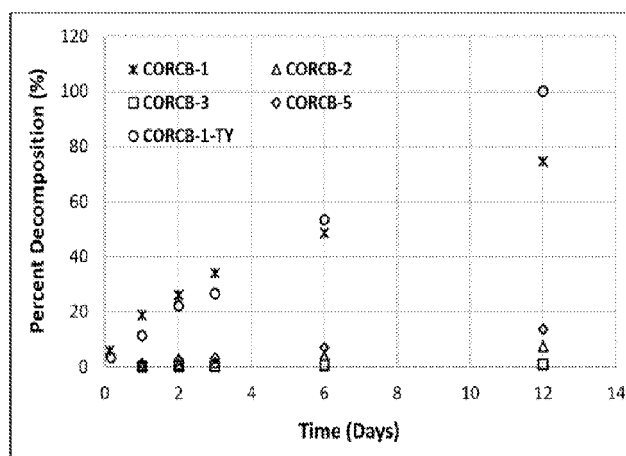
Figure 3. Auto-decomposition of CORCB acid forms monitored by ^1\text{H} NMR. CORCBs were dissolved in \text{D}_2\text{O} and incubated at 37^\circ\text{C} . NMR spectra were taken at specified times to track the decomposition rates.
