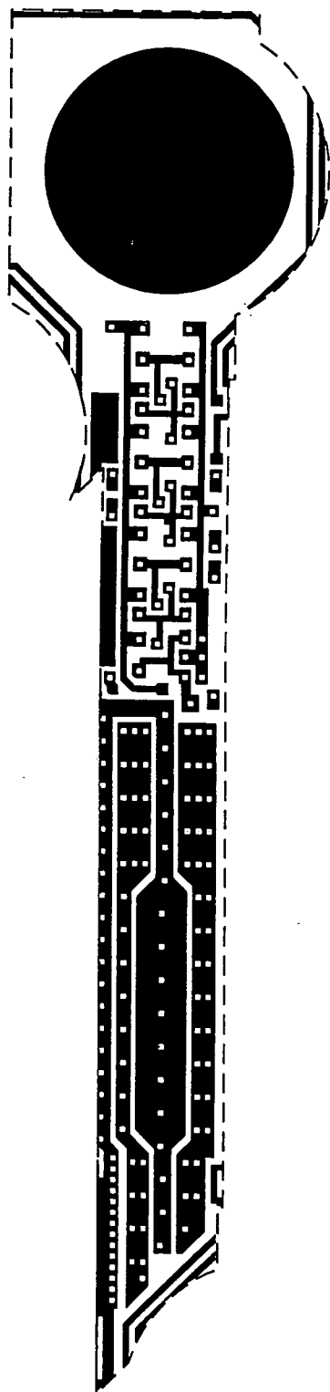
Metal 1 mask
