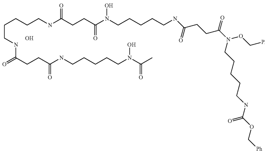
Compound b
