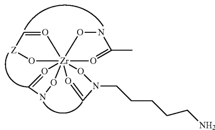
Complex I
