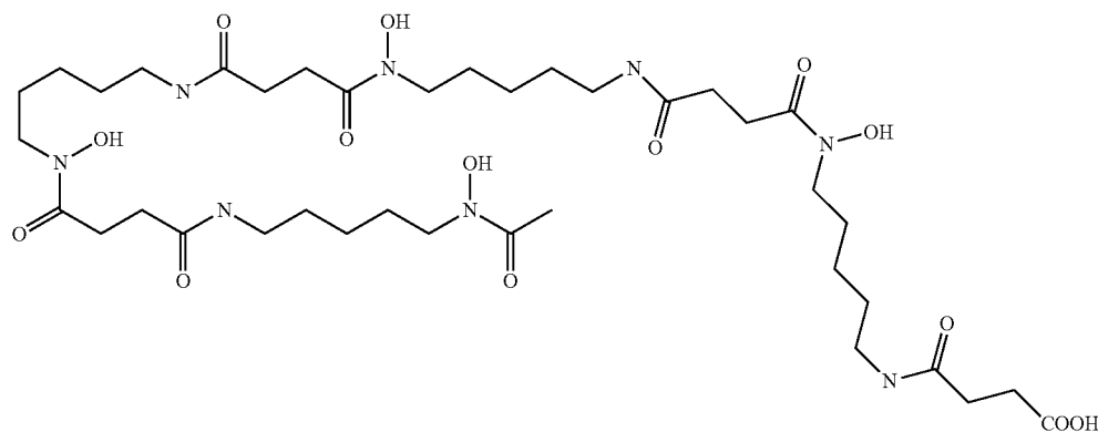
Ligand II
