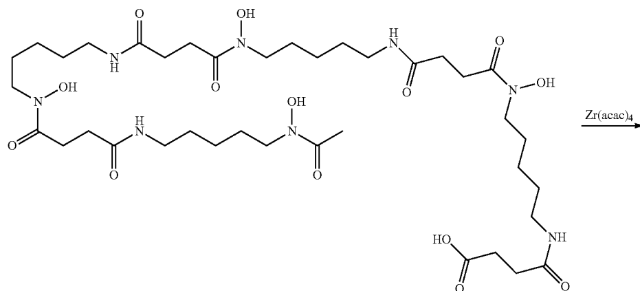
Ligand II
