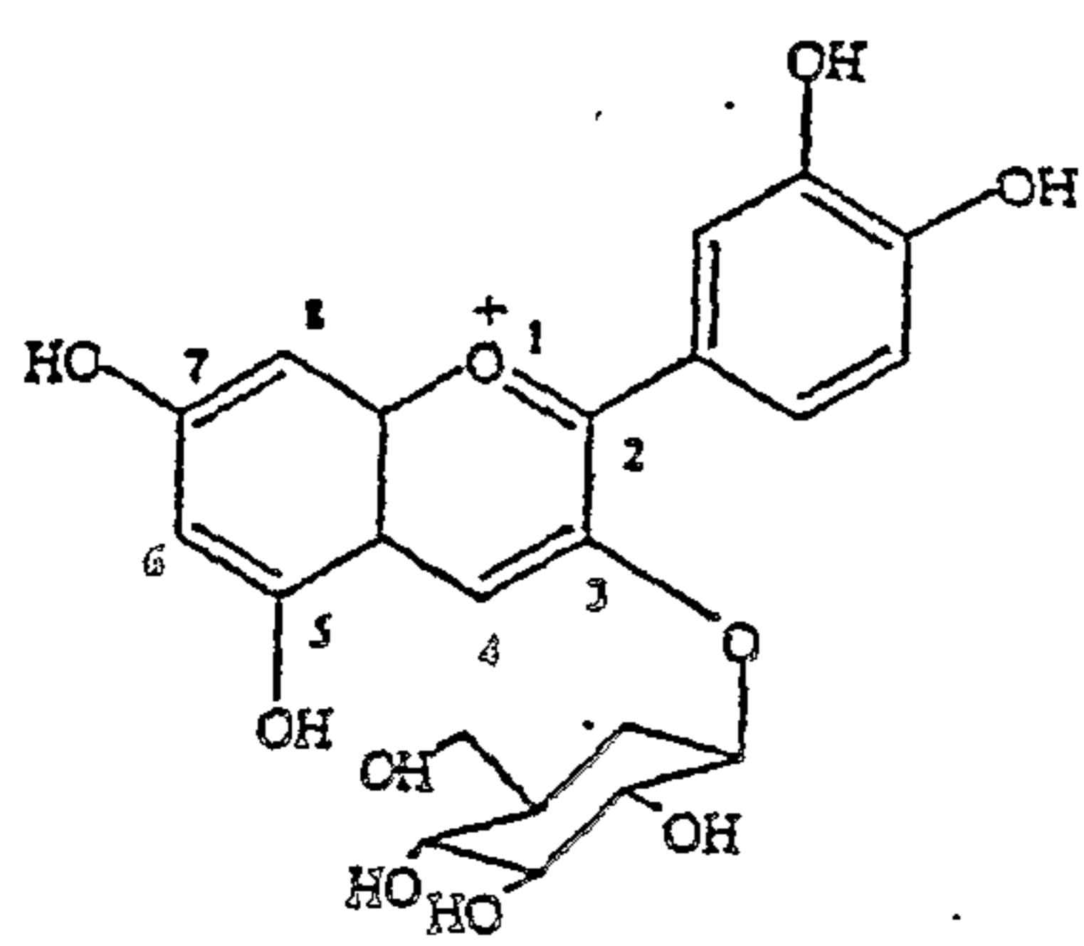
I: Cyanidin-3-glucoside
