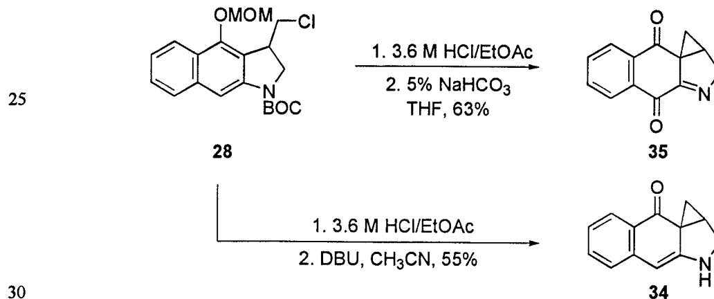
Scheme 4
