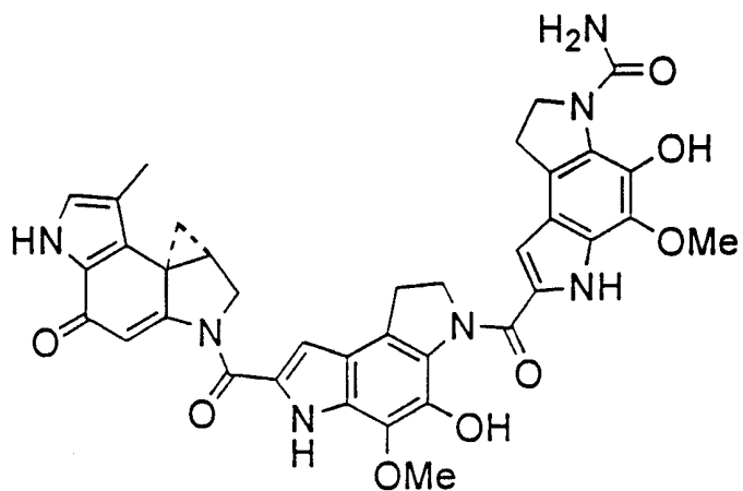
(+)-CC-1065 1
