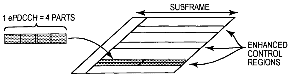
PRIOR ART FIG. 10
