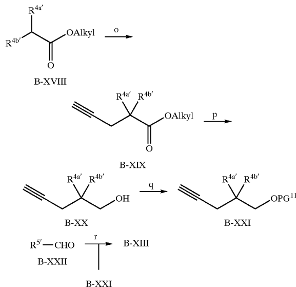
Reaction scheme 5
