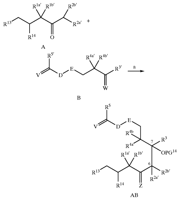
Reaction scheme 8
