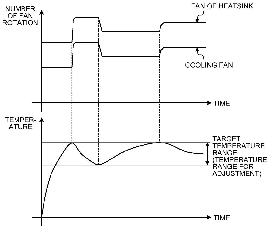
FIG.8C RELATED ART
