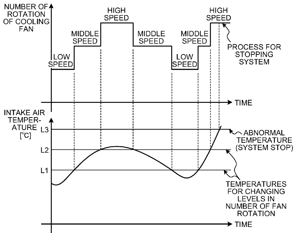
FIG.9C RELATED ART
