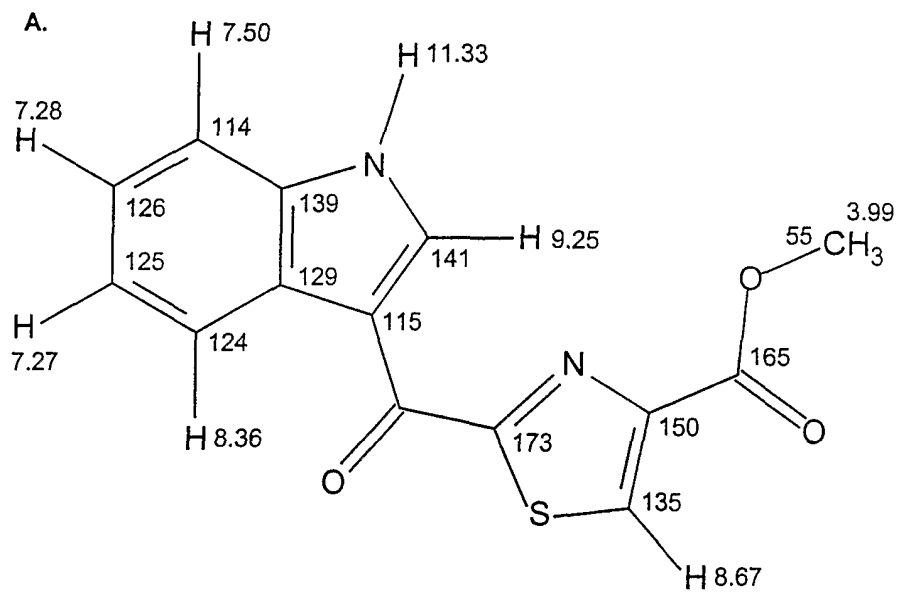
Fig. 7. The Structure of ITE and Dose Responses of ITE and \beta NF
