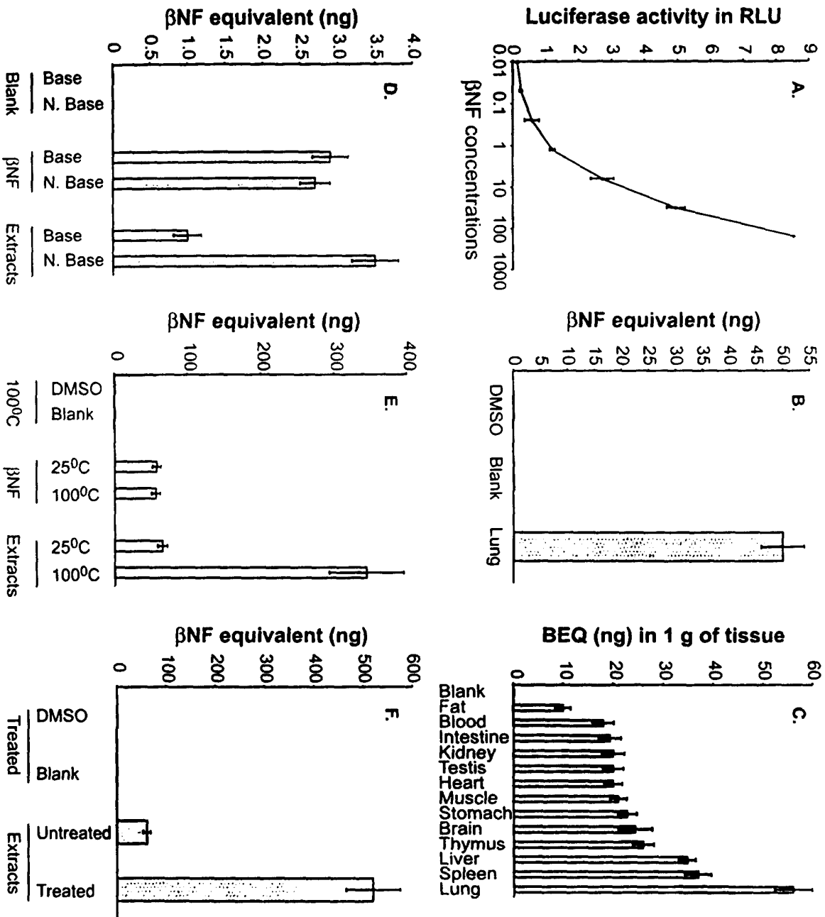
Fig. 1. Reporting Cell Response to βNF and Tissue Extracts
