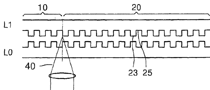
FIG. 3 (PRIOR ART)
