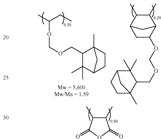
Resist Polymer 4
