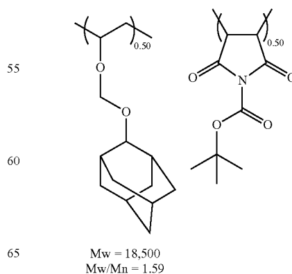
Resist Polymer 1
