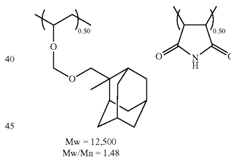
Resist Polymer 5
