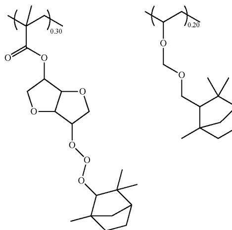
Resister Polymer 9
