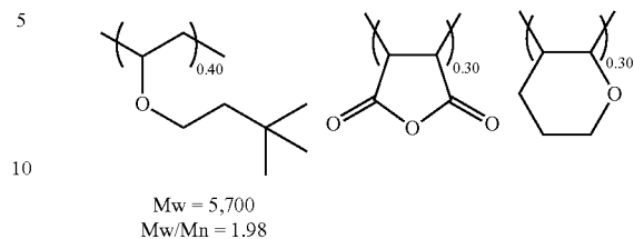
Resist Polymer 3
