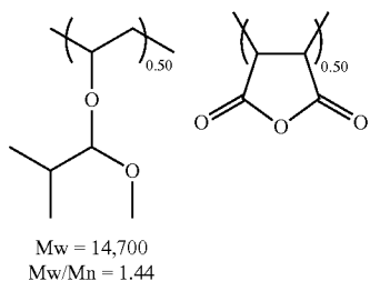
Resist Polymer 6
