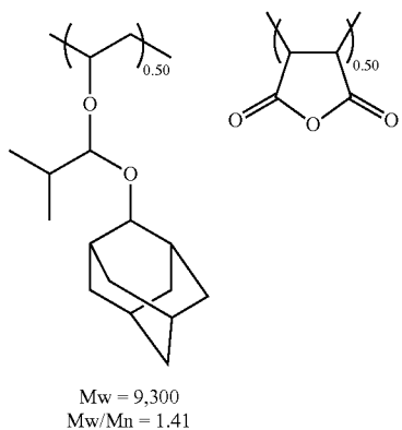
Resist Polymer 7
