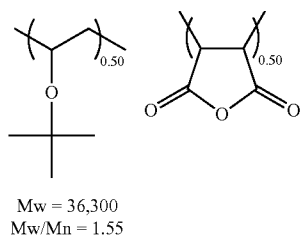
Resist Polymer 1
