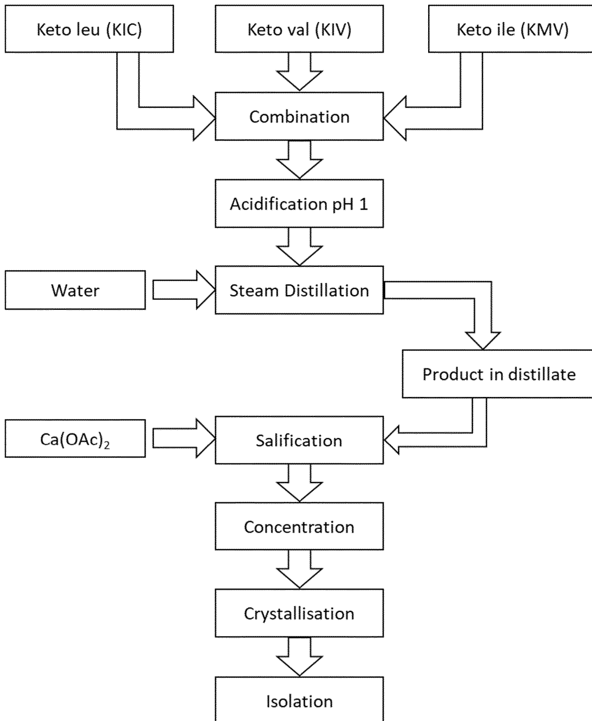
Fig. 1: Co-distillation and co-crystallisation of approximate 2:1:1 keto leucine : keto valine : keto isoleucine calcium salts
