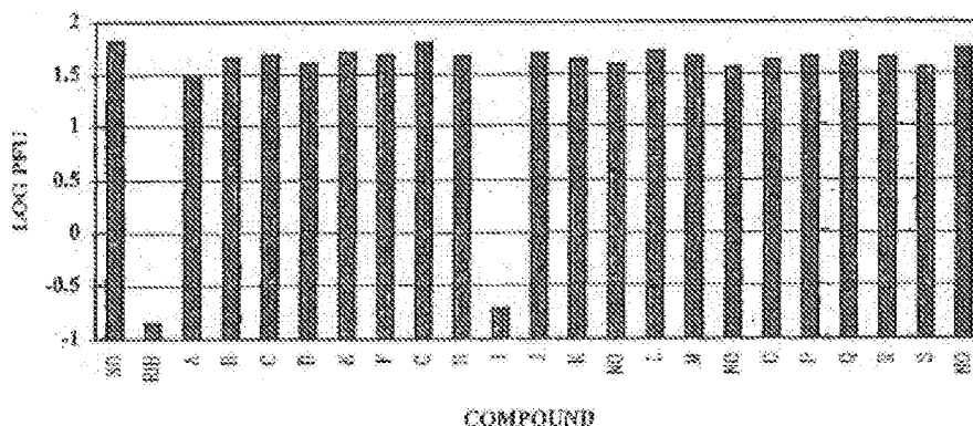
Figure 3: Anti-BVDV compound screening (40 \mu M) in MDEK cells
