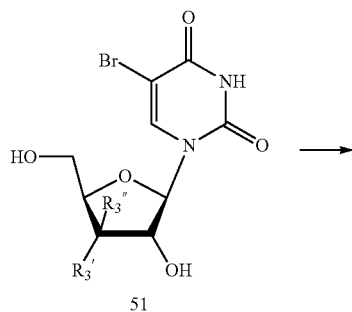
Scheme 15
