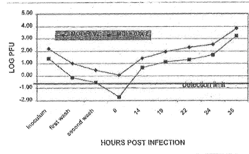
Figure 2: Growth dynamics of BVDV in MDEK cells
