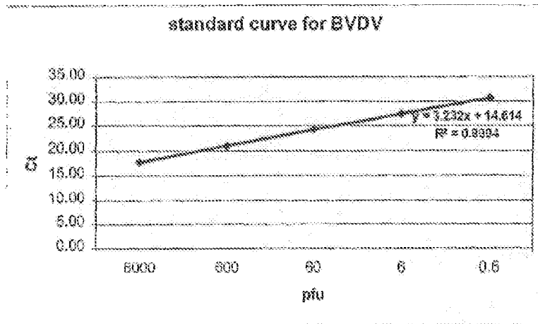
Figure 1: Standard curve for BVDV
