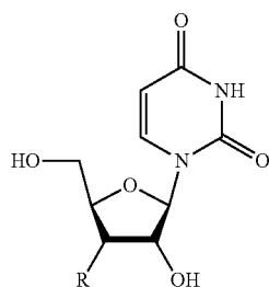
Scheme 9
