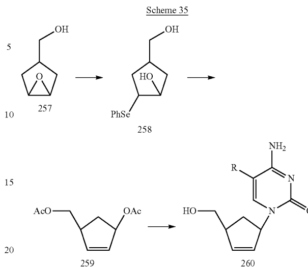
Scheme 36 shows the synthesis of 3,4-unsaturated carba nucleoside of type VII Wolfe et al ( J. Org. Chem. , 1990, 55,
