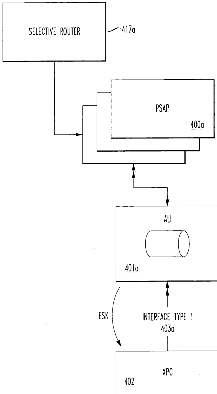
FIG. 4 (PRIOR ART)
