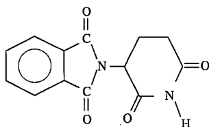
thalidomide
