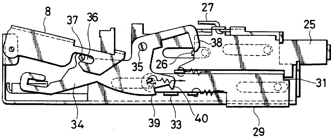
FIG. 11 PRIOR ART
