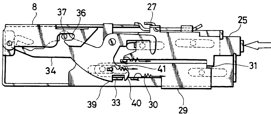
FIG.12 PRIOR ART
