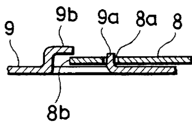
FIG.13 PRIOR ART
