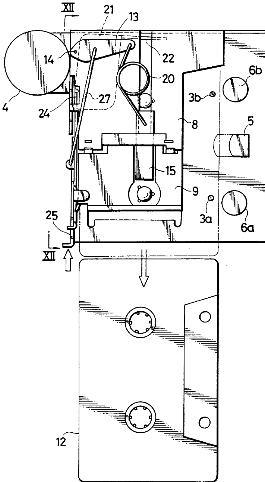
FIG. 7 PRIOR ART
