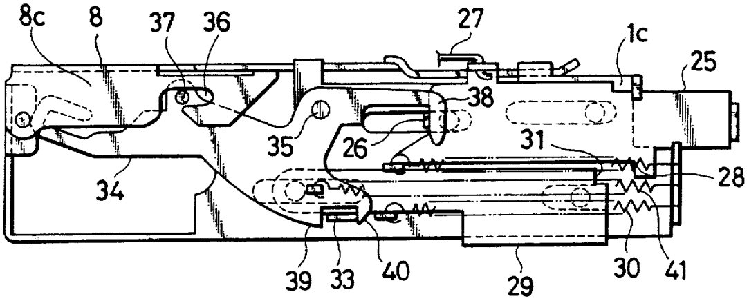
FIG. 10 PRIOR ART
