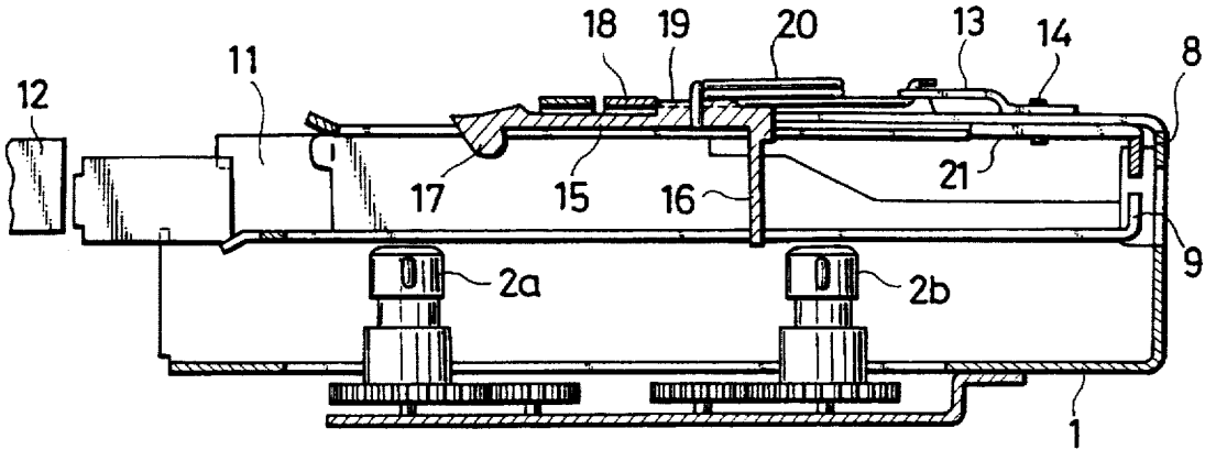
FIG. 8 PRIOR ART
