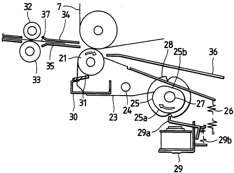
FIG. 8 (PRIOR ART)
