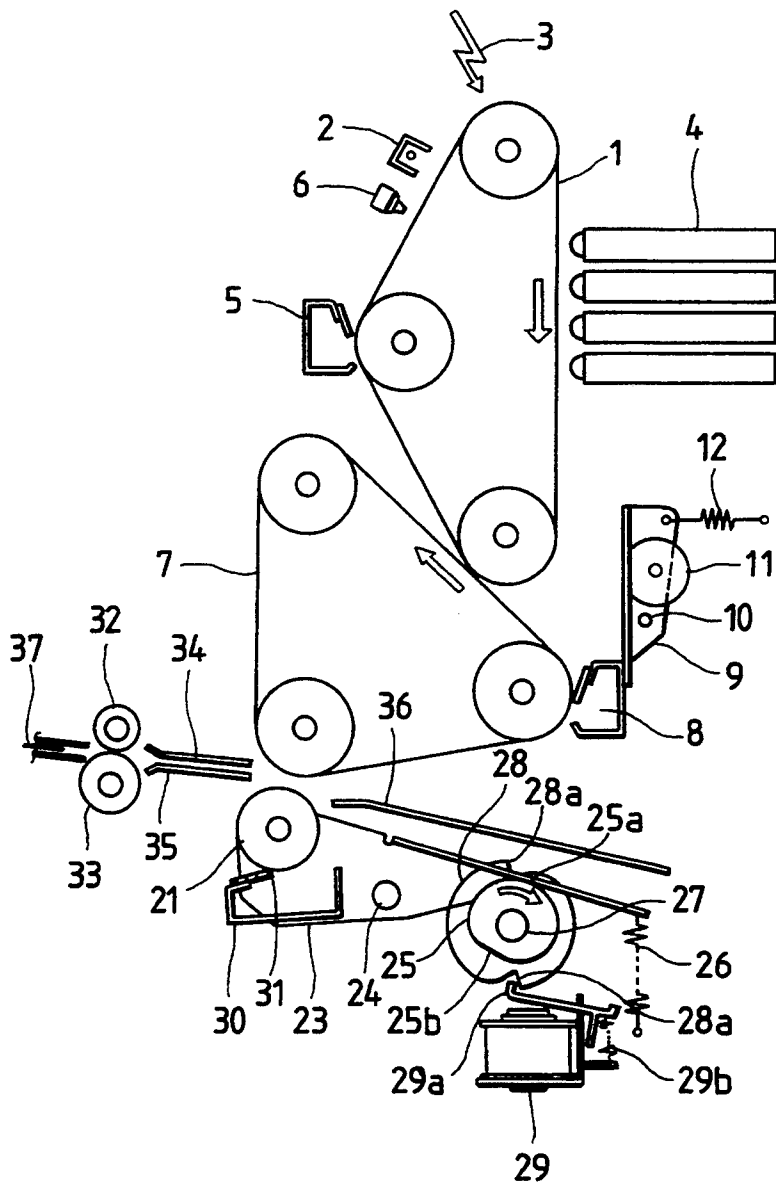
FIG. 7 (PRIOR ART)
