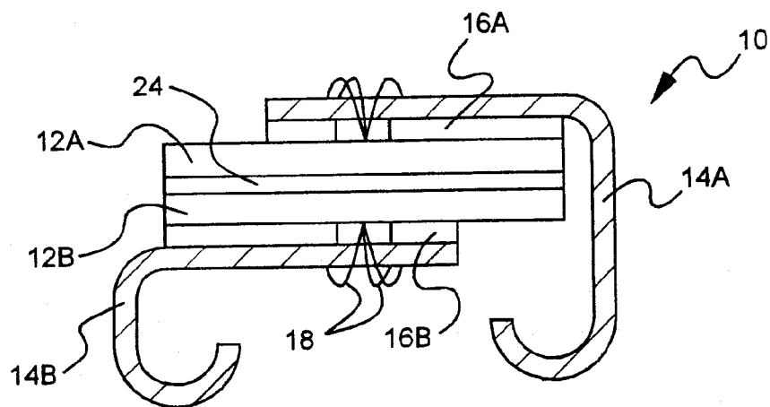
FIG. 7 (PRIOR ART)
