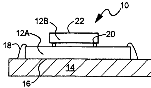
FIG. 3 (PRIOR ART)
