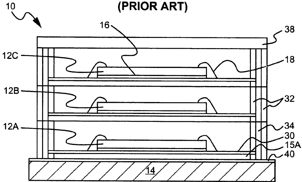
FIG. 10 (PRIOR ART)
