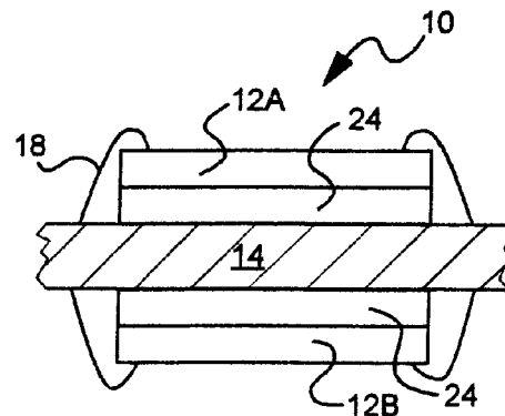
FIG. 6 (PRIOR ART)
