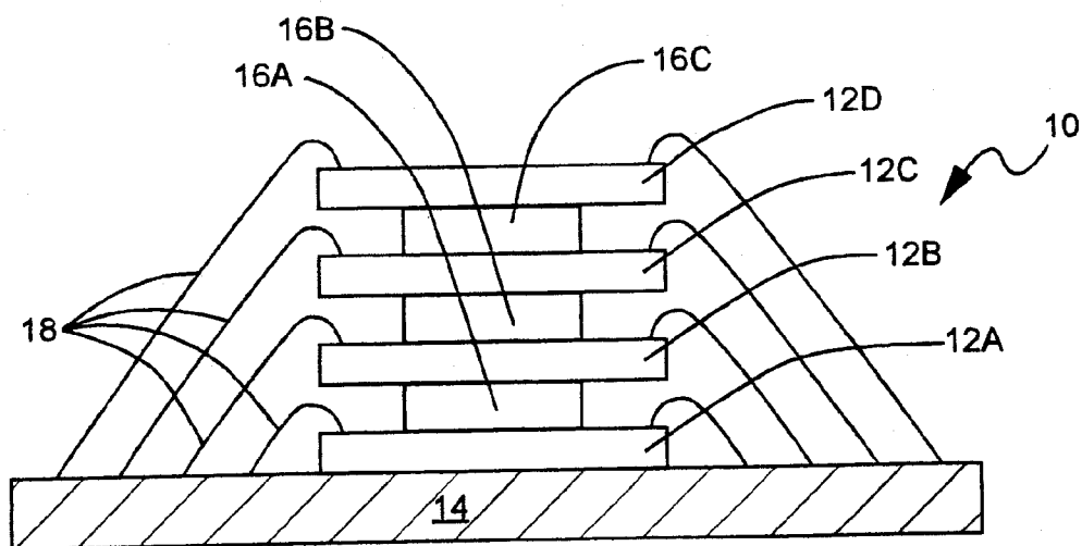
FIG. 8 (PRIOR ART)
