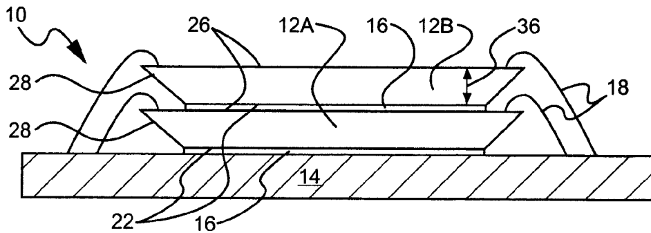
FIG. 11 (PRIOR ART)
