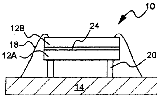
FIG. 5 (PRIOR ART)
